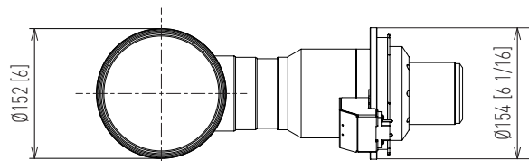
ET-D3LEU100
