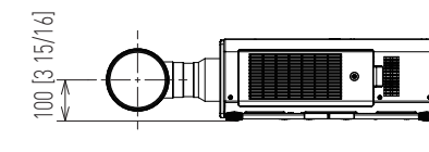
ET-D3LEU100+PT-DZ13K/PT-DS12K/PT-DW11K/PT-DZ10K
