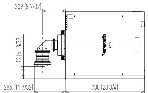
ET-D3LEU100+PT-RQ22K/PT-RZ21K/PT-RS20K
