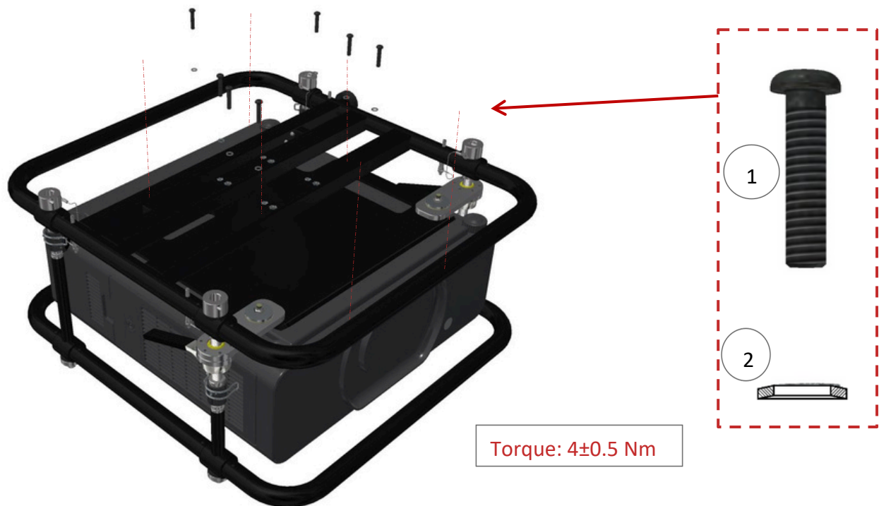
Figure 5 Securely tighten all screws
