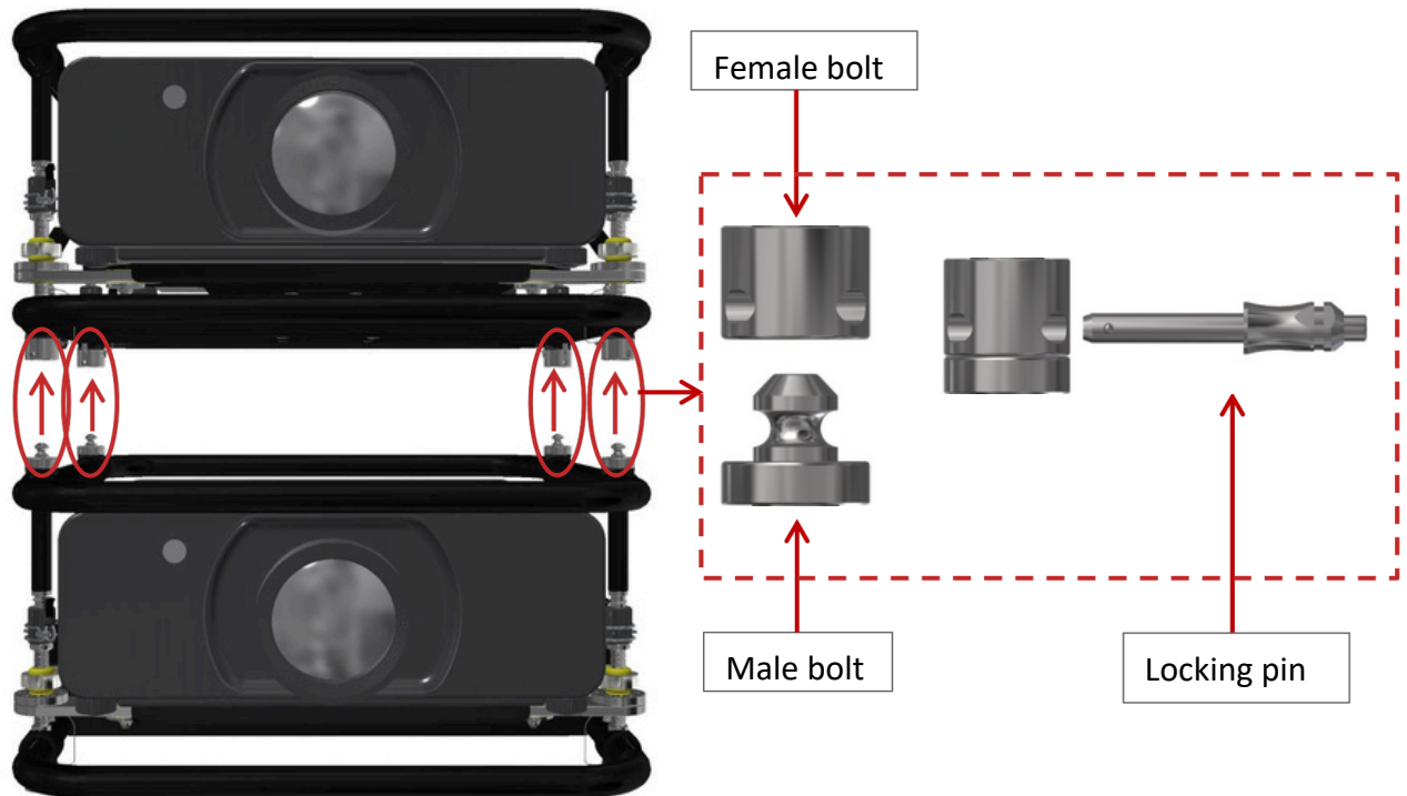
Figure 20 Stacking frames
