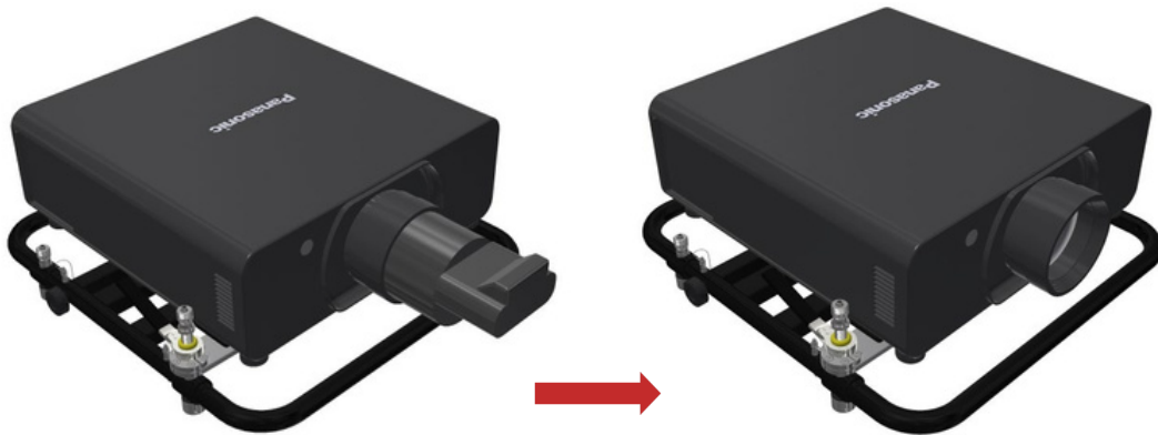
Figure 12 Remove the ultra-short throw lens
