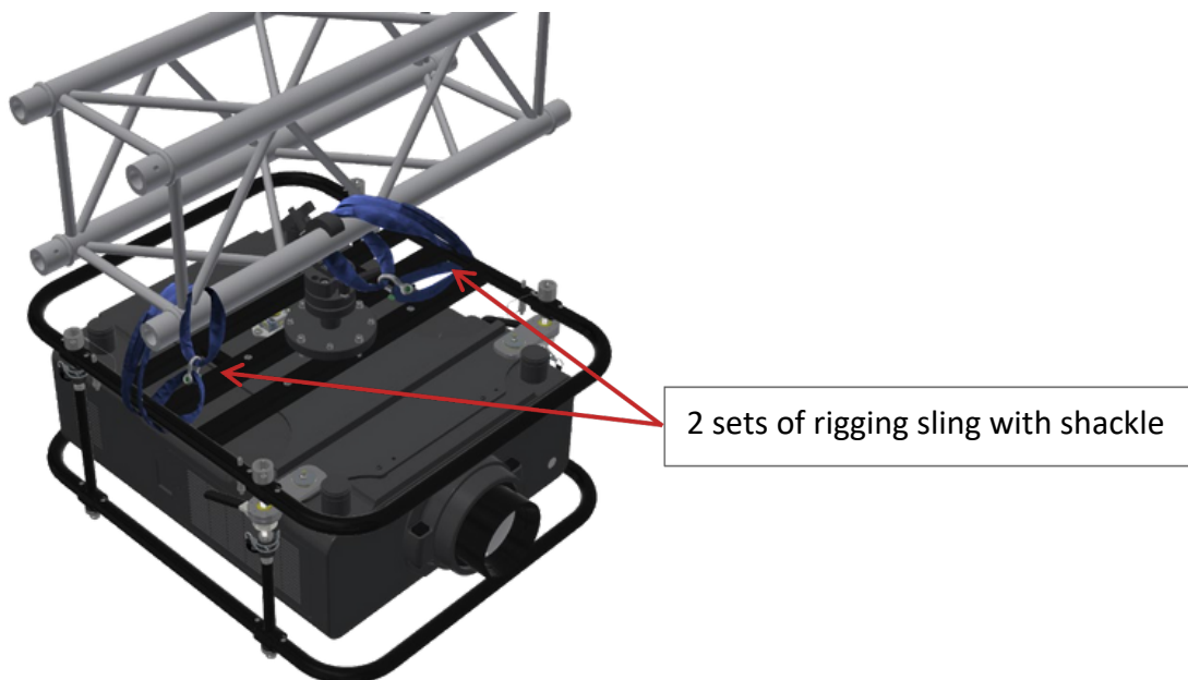
Figure 23 Securing one frame with two sets of rigging slings
