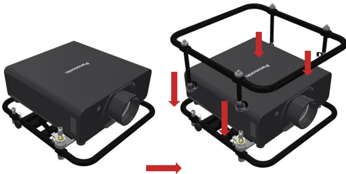
Figure 13 Reposition the upper ring
