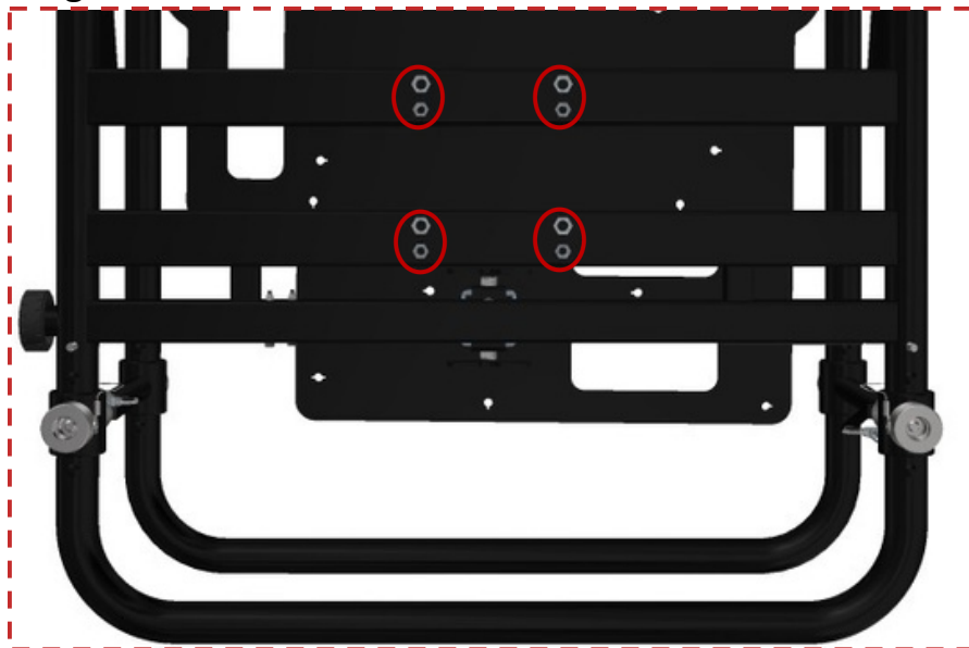
Figure 25 Inspection of mounting threads at bottom side
