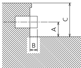
Sectional view of terminal b (USB/DVI-D OUT/DVI-D IN/HDMI 1,2/DIGITAL LINK LAN/PC IN)
