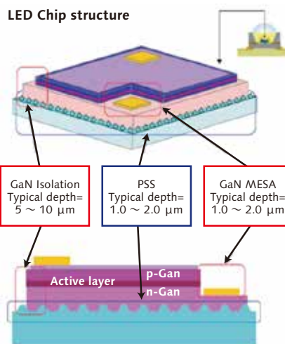
GaN processing
