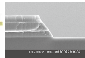
GaN processing
