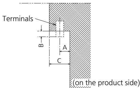
Sectional view of terminal a (AUDIO OUT / AUDIO IN / VIDEO AV IN / SERIAL IN / PC IN / DVI-D IN)
