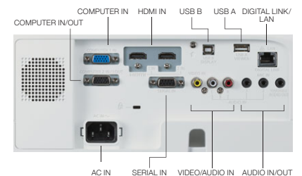
Terminal layout for PT-VZ575N/VW535N/VX605N.
