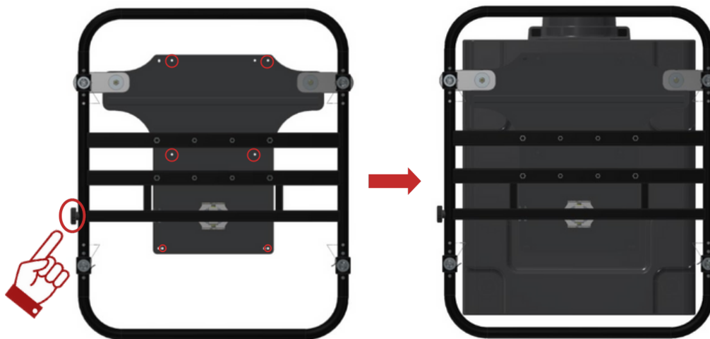
Figure 4 Mounting the projector into the frame
