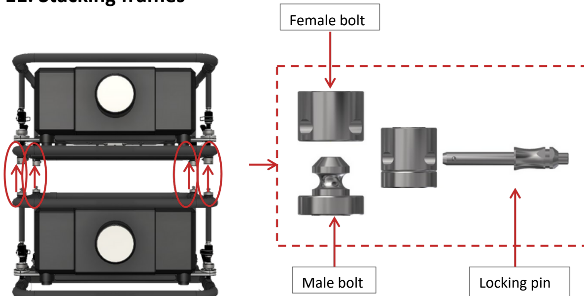
Figure 20 Stacking frames
