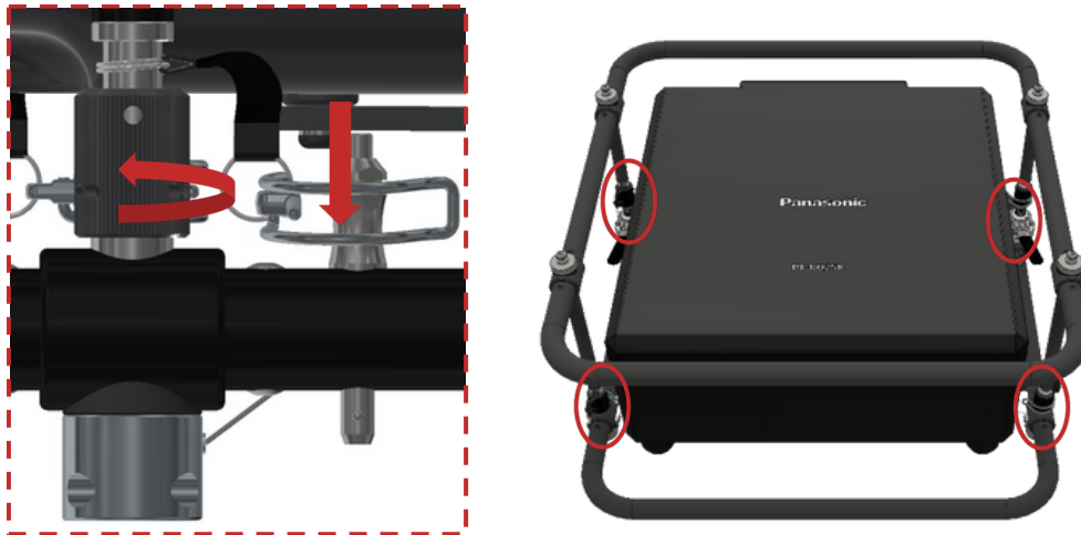
Figure 14 Tighten the four attachment nuts
