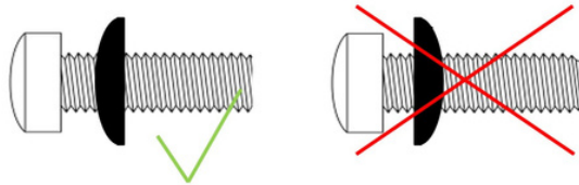
Figure 6 Orientation of Schnorr safety washer
