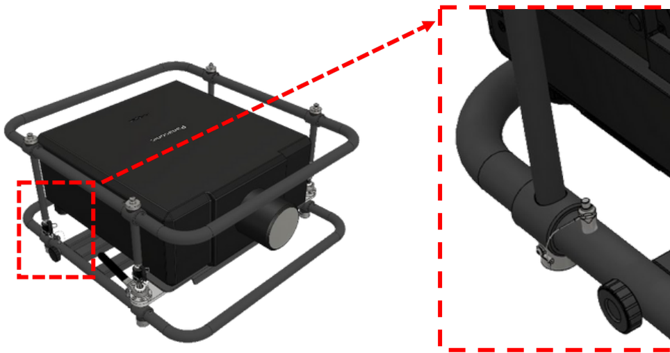
Figure 30 Locking pins at the frame
